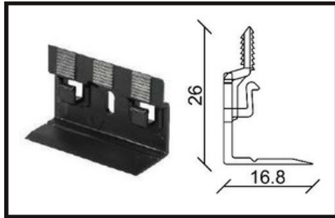
CLIPHOLDER for skirting boards Structure: Plastic
